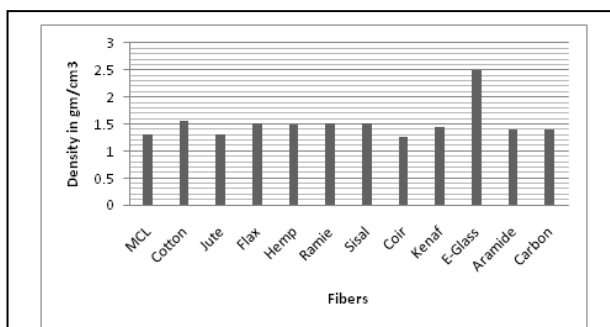
Fig. 6: Comparison of density of MCL with other fibers
