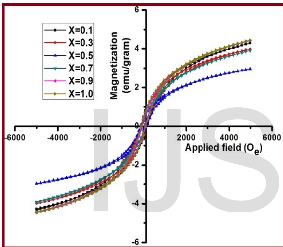
Figure 5(a-f): Magnetic hysteresis loops for NiCr x Fe 2-x O 4 nano ferrites
