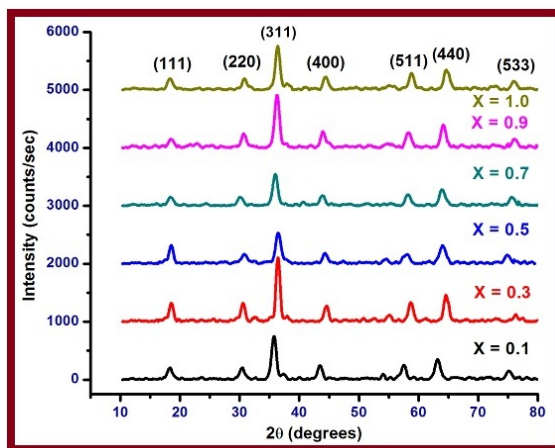
Figure 1: X-ray diffraction pattern of mixed \text{NiCr}_x\text{Fe}_{2-x}\text{O}_4 nano ferrites
