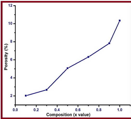
Figure 3: Porosity variation with Cr concentration
