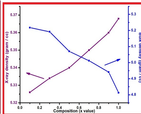
Figure 2: X-ray density and bulk density variation with Cr concentration
