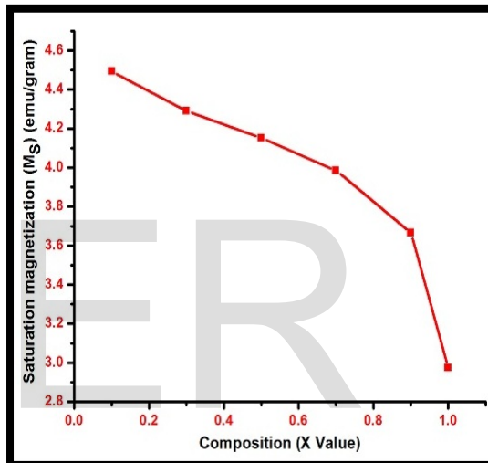
Figure 6: Variation of saturation magnetization with Cr concentration
