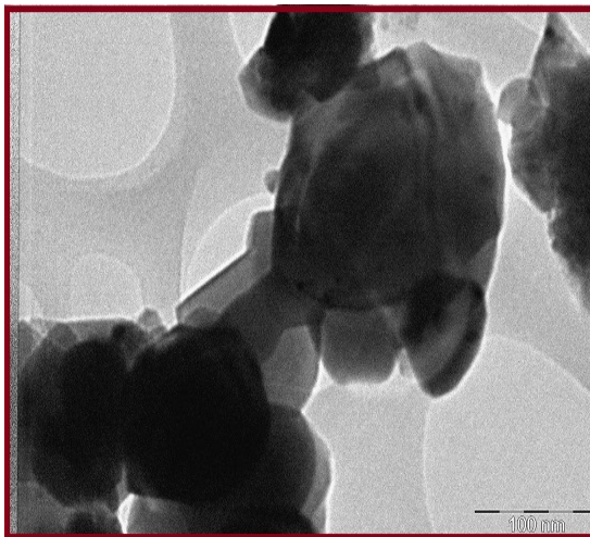
Figure 4: TEM images of NiCr 0.7 Fe 1.3 O 4 nano ferrite
