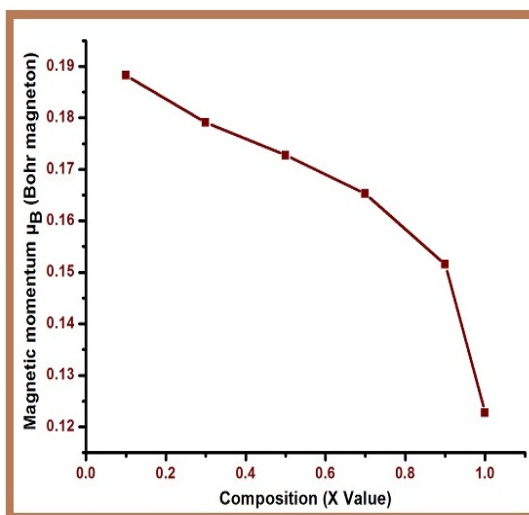
Figure 7: Variation of magnetic moment with Cr concentration
