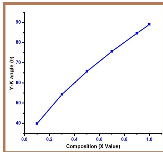
Figure 8: Variation of Y-K angle with Cr concentration
