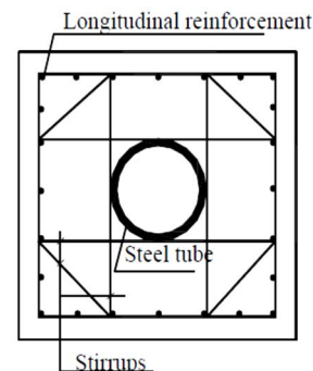
Fig.1 Encased composite column
