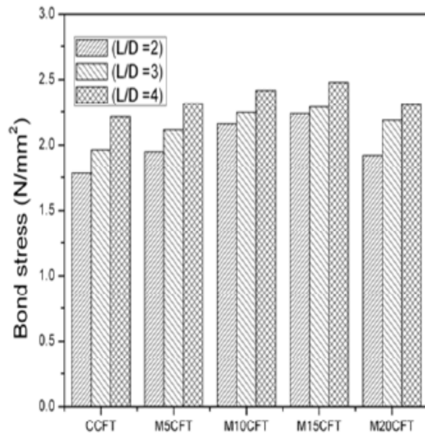
Fig 4. Bond stress of CFT and MCFT
