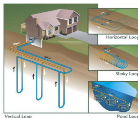
Fig. 1: Residential Ground Loops [24]
