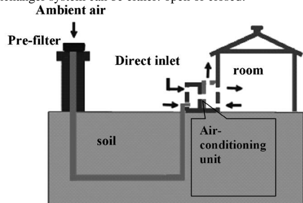
Fig. 2: Basic principle of ground preheating or pre-cooling of air in an open system [8]
