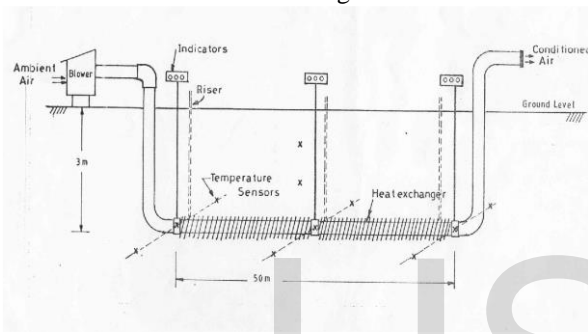
Fig. 5: Earth tube Heat Exchanger [9]
