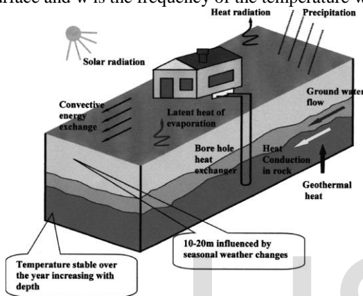
Fig. 3: Energy flows of ground [8]
