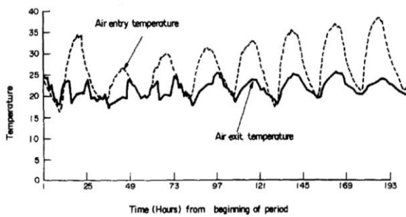
Fig. 4: Entry and Exit air temperature[3]
