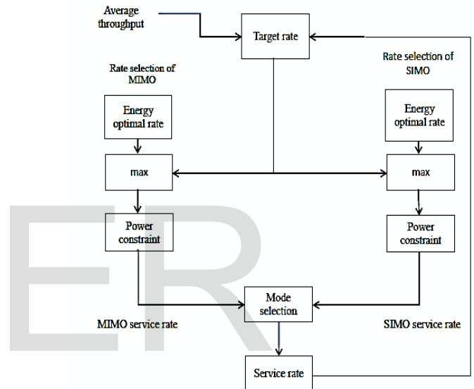
Figure 1. Flow chart of the CUTE algorithm.
