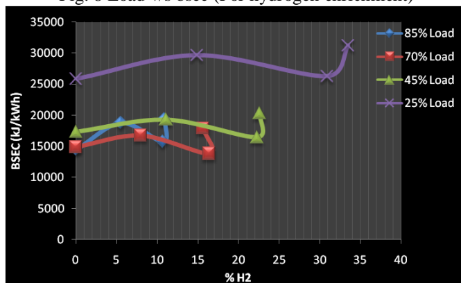
Fig. 8 Load v/s bsec (For hydrogen enrichment)
