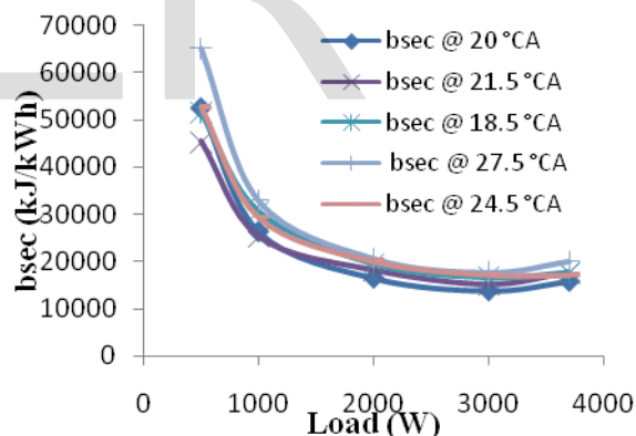
Fig. 8 Load v/s bsec (For hydrogen enrichment)
